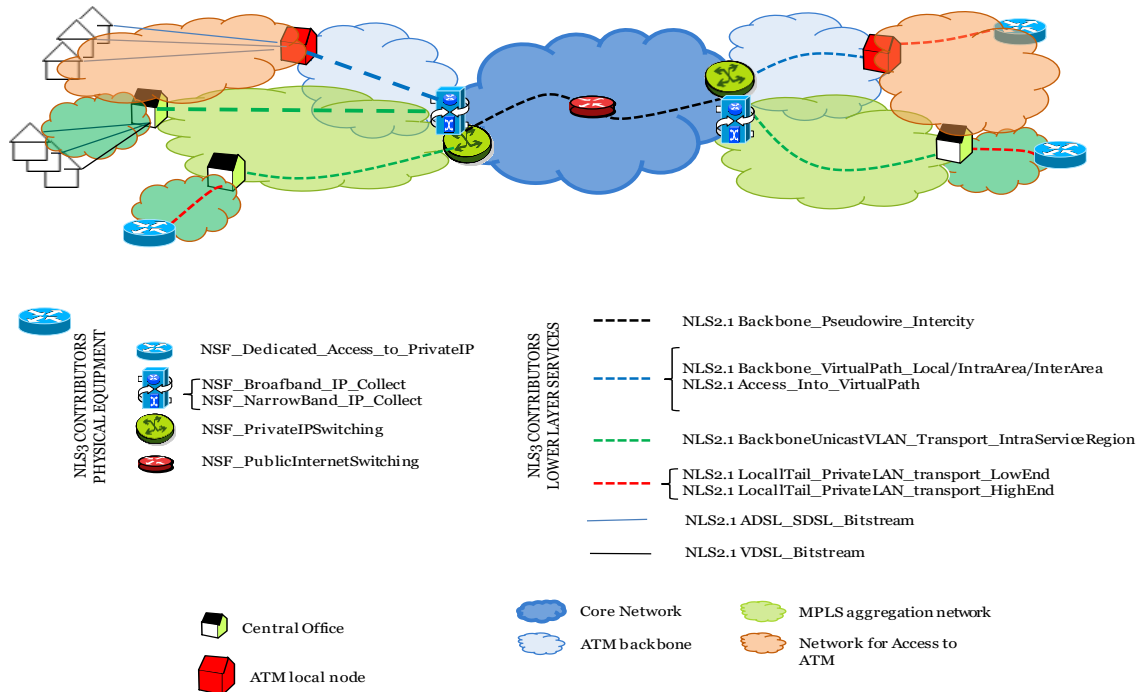
Figure 10: Layer 3 topology and contributors
